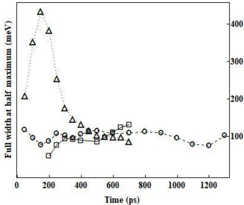
Fig. 2. Time dependence of the width of the maximum of the fitting function at \epsilon = \epsilon_x (circles), \epsilon = \epsilon_{xx} (squares), and \epsilon = \epsilon_{xxx} (triangles).
