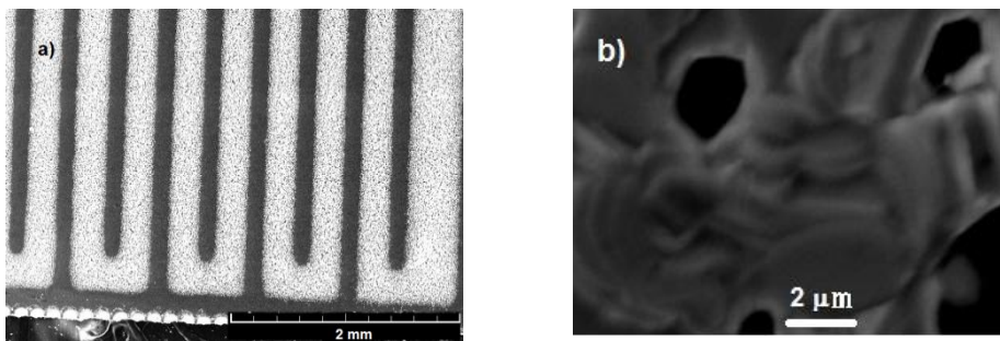
Fig. 1. (a) SEM of an \text{As}_2\text{Te}_{13}\text{Ge}_8\text{S}_3 film with interdigital Pt electrodes and (b) the morphology of the ChGS surface magnified by 10^3 times.
