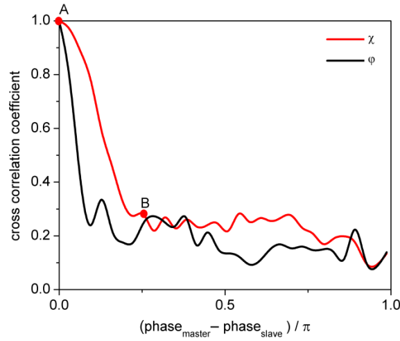
Fig. 2. Cross-correlation coefficient as a function of the feedback phase difference (phase master – phase slave) for coupling \zeta = 20 . Parameters: \phi_s = 0 , \psi_m = \psi_s = \pi/5 , \chi_s = 0 , \theta_m = \theta_s = \pi/4 .
