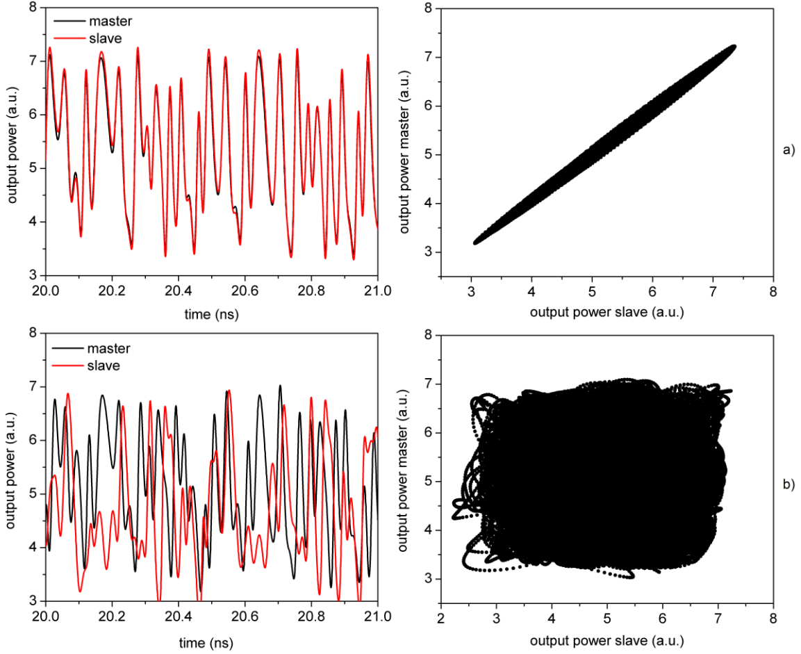
Fig. 3. Pulse traces of output power (left) and synchronization diagram (right) for points A (a) and B (b) of Fig 2. Parameters are the same as in Fig. 2.
