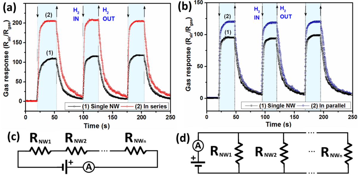
Fig. 4. (a) Gas response of a single NW and two Pd/ZnO NWs connected in series to 100 ppm \text{H}_2 gas (diameter D \approx 160 nm and length L \approx 1 \mu\text{m} ). (b) Gas response of a single NW and two Pd/ZnO NWs connected in parallel to 100 ppm \text{H}_2 gas ( D \approx 190 nm and L \approx 1.3 \mu\text{m} ). Schematics of the sensor structure based on individual Pd/ZnO NWs connected: (c) in series; and (d) in parallel.
