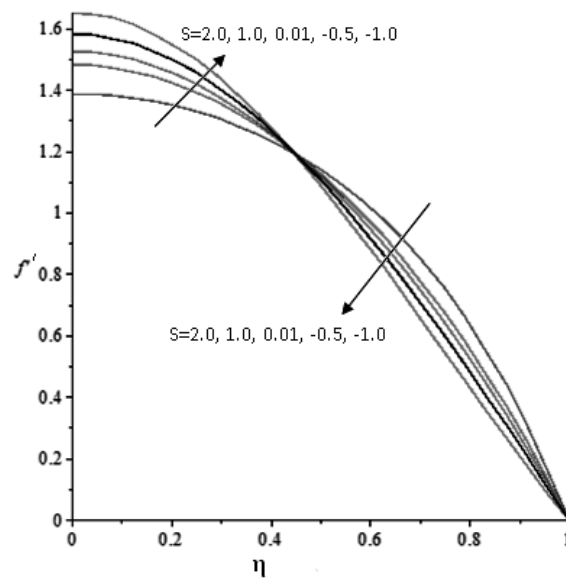
Fig. 4. Velocity profiles for various S values.
