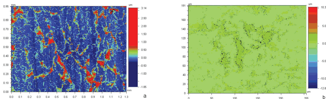
Fig. 6. Modification in the roughness of the epoxy resin/ \text{TiO}_2 (anatase) 1% composite caused by \gamma -irradiation in water: nonirradiated sample and (b) 20 kGy.
