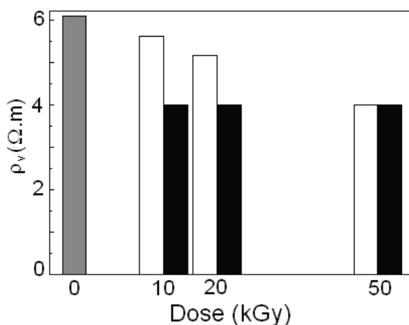
Fig. 4. Resistivity of unmodified epoxy resin subjected to \gamma -irradiation. (grey) pristine material; (white) irradiation in air; and (black) irradiation in water.
