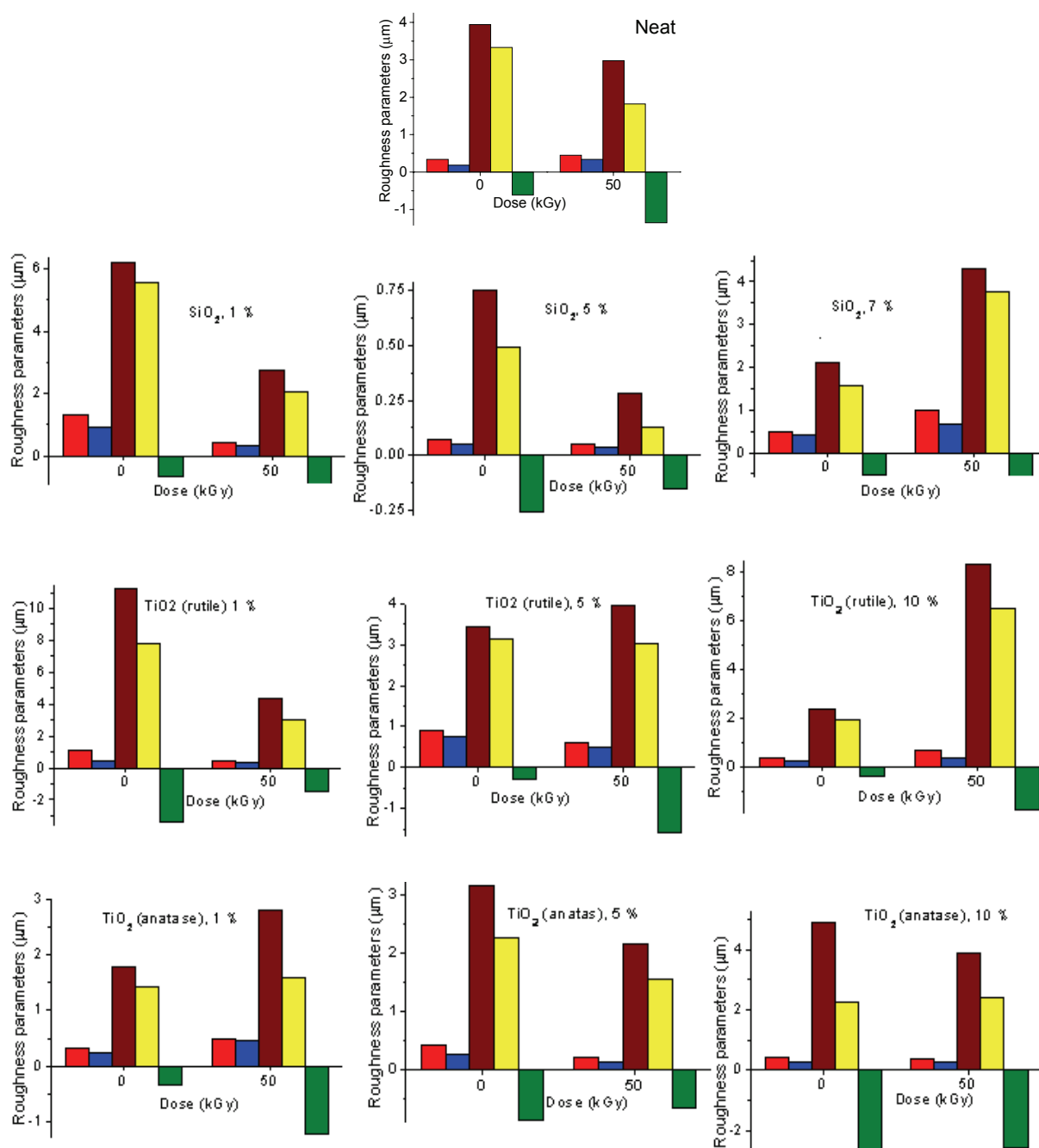
Fig. 8. Changes in the roughness parameters assessed for \gamma -irradiated epoxy resin/filler nano-composites.
