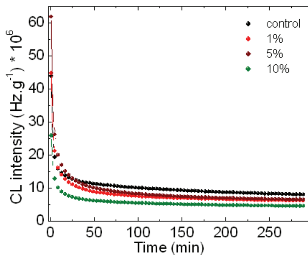
Fig. 2. CL curves for oxidation of \gamma -irradiated epoxy resin/TiO 2 nanocomposite. Received dose is 50 kGy.
