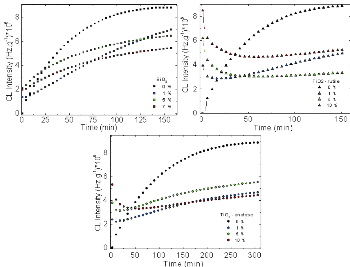
Fig. 1. CL curves depicting the progress of oxidation on epoxy resin nanocomposites.
