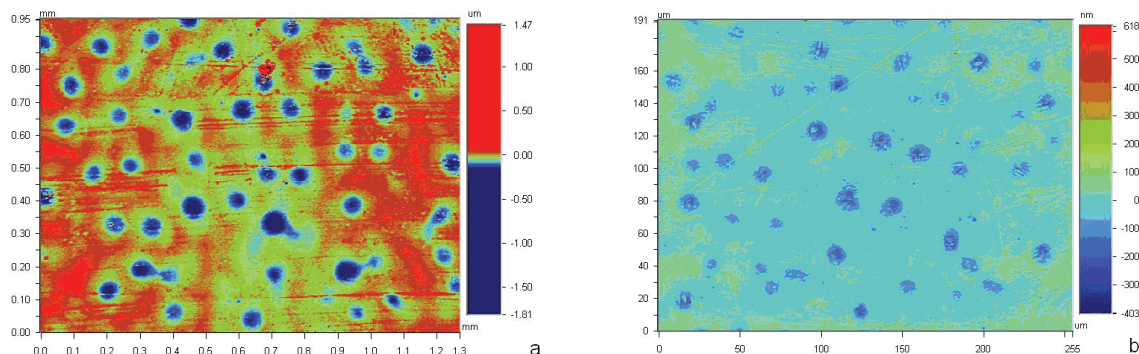
Fig. 7. Modification in the roughness of the epoxy resin/ \text{SiO}_2 5% composite caused by \gamma -irradiation: (a) nonirradiated sample and (b) 20 kGy in water.
