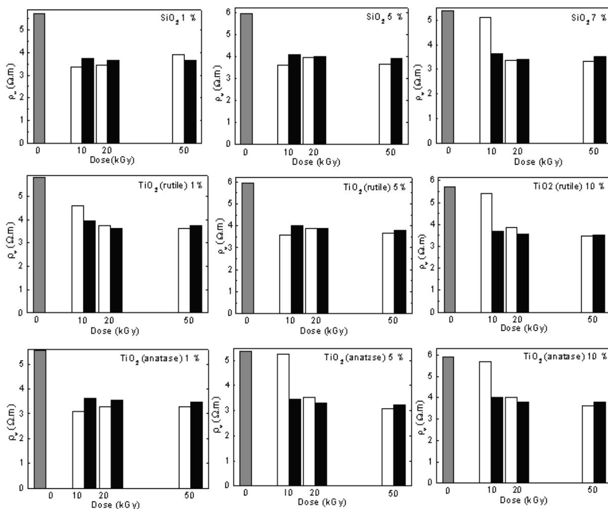
Fig. 5. Volume resistivity of radiation processed epoxy resin nanocomposites.
