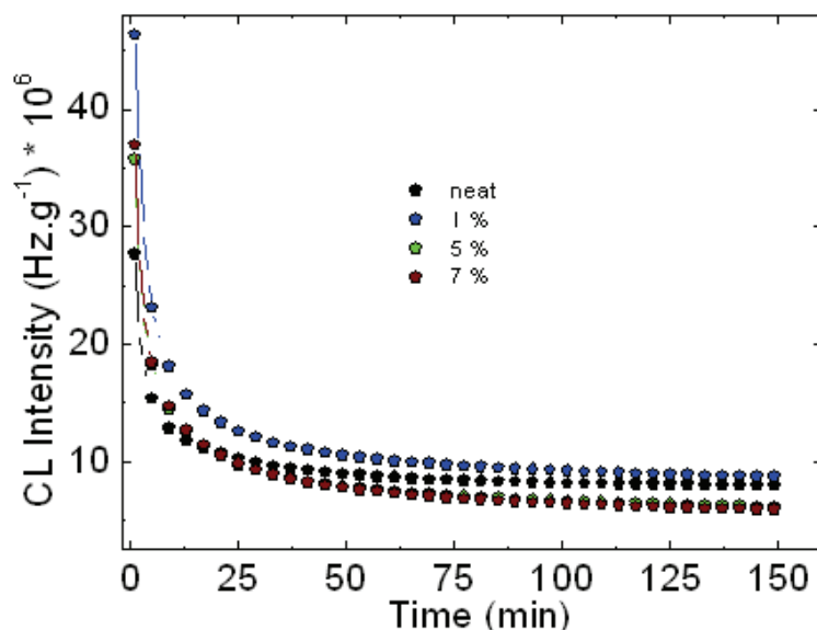
Fig. 3. CL curves for oxidation of \gamma -irradiated epoxy resin/SiO 2 nanocomposite. Received dose is 50 kGy.
