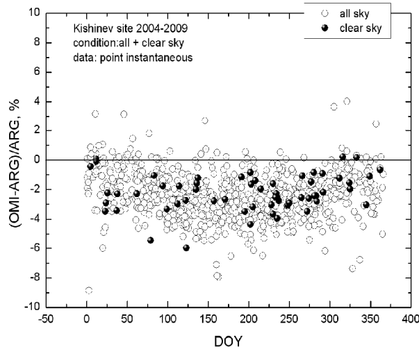
Fig. 4. Intra-annual variability of relative difference (\text{OMI-ARG})/\text{ARG} (in %) versus day of year (DOY). Case of instantaneous OMI overpass and ARG ground TOC observations for all sky and for clear sky conditions. Period of observation: October 2004 to November 2009.
