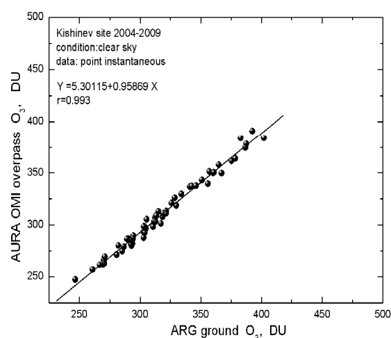
Fig. 2. Scatter plot of OMI overpass versus ARG ground TOC data from instantaneous observations for clear sky conditions. The equation of regression line (solid line) is indicated. Period of observation from October 2004 to November 2009.
