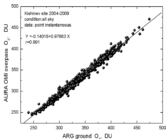
Fig. 1. Scatter plot of OMI overpass versus ARG ground TOC data from instantaneous observations for all sky conditions. The equation of regression line (solid line) is indicated. Period of observation from October 2004 to November 2009.
