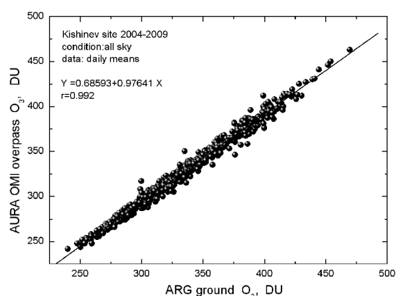
Fig. 3. Scatter plot of OMI overpass TOC daily means versus ARG ground TOC daily averages from observations for all sky conditions. The equation of regression line (solid line) is indicated. Period of observation from October 2004 to November 2009.
