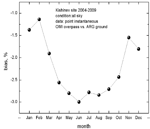
Fig. 5. Seasonal variability of multiyear means of relative difference b (in %) versus month. Case of instantaneous OMI overpass and ARG ground TOC observations for all sky conditions. Period of observation: October 2004 to November 2009.
