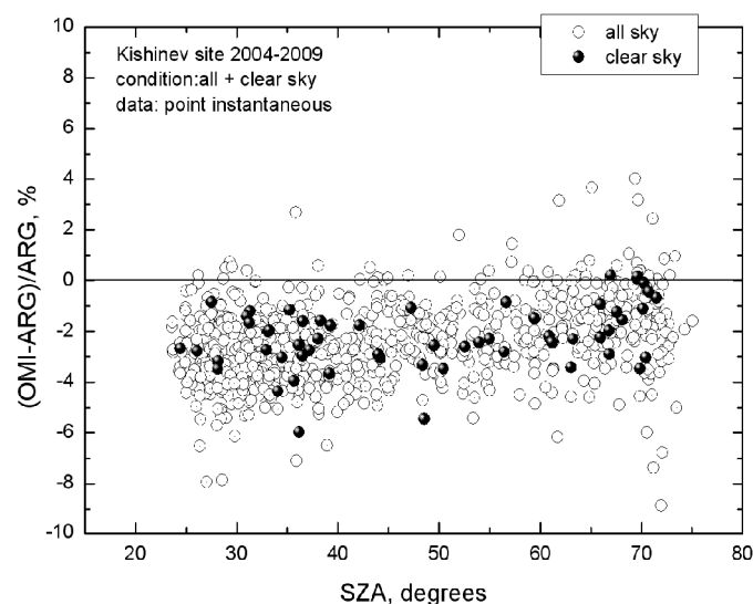
Fig. 6. Variability of relative difference (\text{OMI-ARG})/\text{ARG} , (in %) versus solar zenith angle (SZA). Case of instantaneous OMI overpass and ARG ground TOC observations for all sky and for clear sky conditions. Period of observation: October 2004- November 2009.
