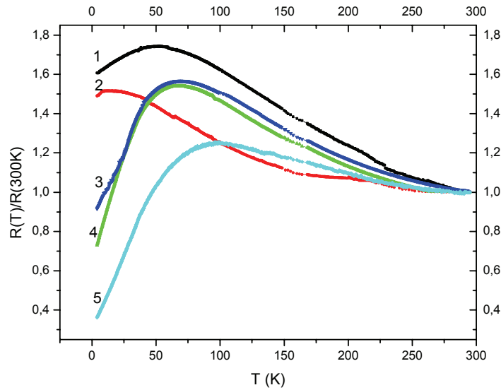
Fig. 2. Temperature dependence of resistance normalized to the resistance at 300 K for as-prepared Bi NWs: (1) d = 90 nm, (3) d = 120 nm and thermally annealed: (2) d = 90 nm, (4) d = 120 nm, (5) d = 150 nm.
