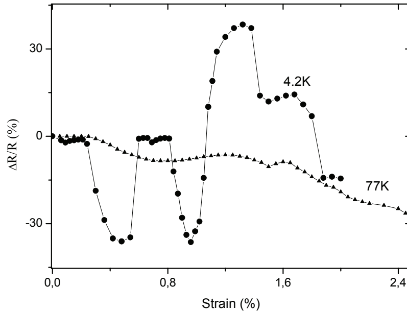
Fig. 1. Relative variation of the resistance as a function of applied strain for a 90-nm Bi nanowire measured at 4.2 K and 77 K.
